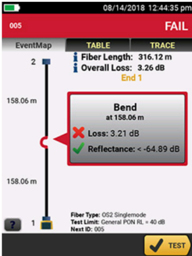
Bend as seen on a EventMap
