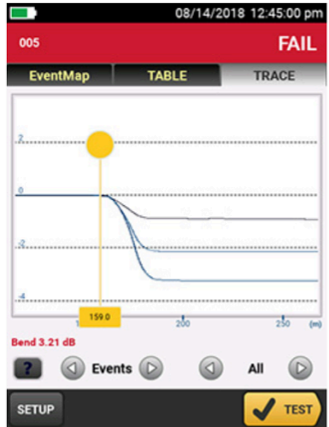
Bend as seen on an OTDR trace
