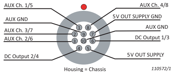
Fig. 6 10-pin LEMO® auxiliary connector
