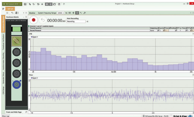
Fig. 3 BK Connect Hardware Setup: Hardware Matrix (graphical representation of a LAN-XI front end) and Monitor
