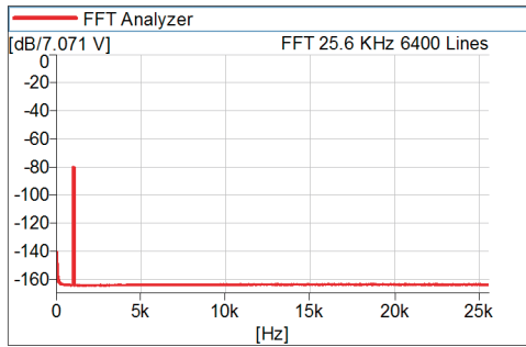
Fig. 5 160 dB analysis in one range. An FFT measuring a 1 kHz signal 80 dB below full scale ( 7 V_{rms} ). Note that noise and all spurious components measure 160 dB below full-scale input
